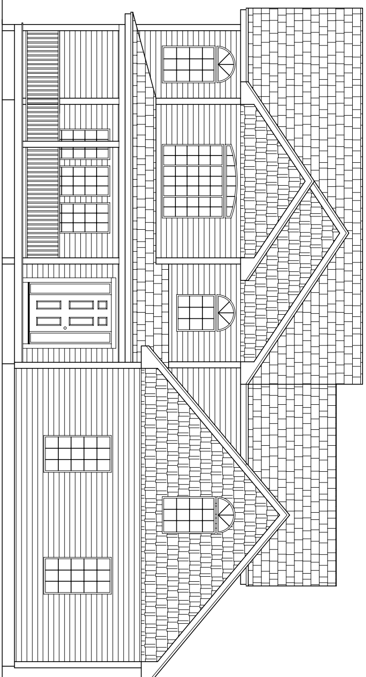
FRONT ELEVATION
